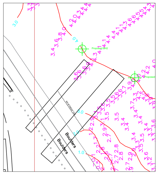
Bathymetry at Proposed Borehole Locations 1:1000
