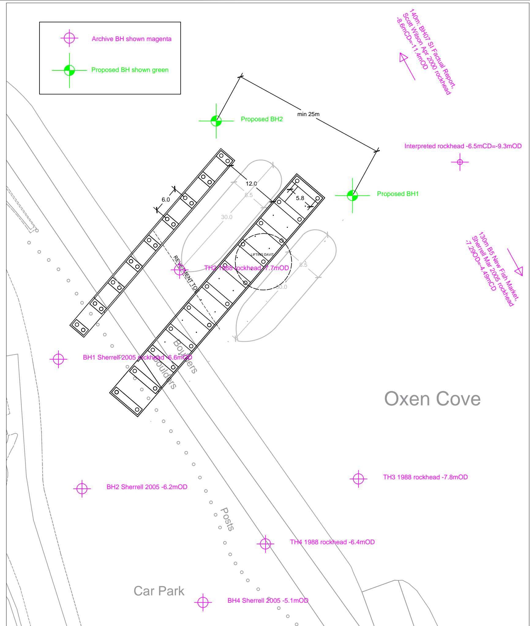
Archive and Proposed Borehole Locations 1:500
